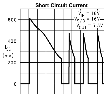
200 \text{ms}/\text{Div} Figure 20.
