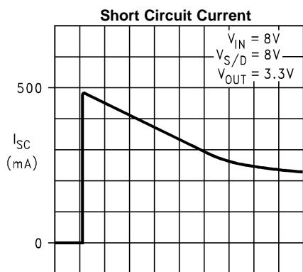
500 \text{ms}/\text{Div} Figure 19.
