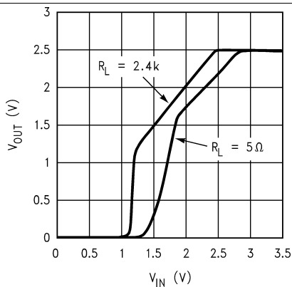
Figure 1. Dropout Characteristics
