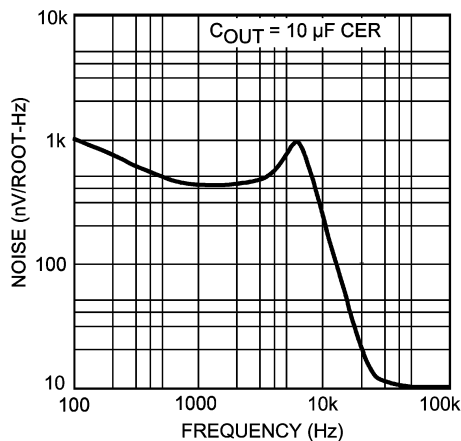
Figure 1. Noise Density
