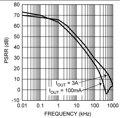
Figure 14. PSRR
