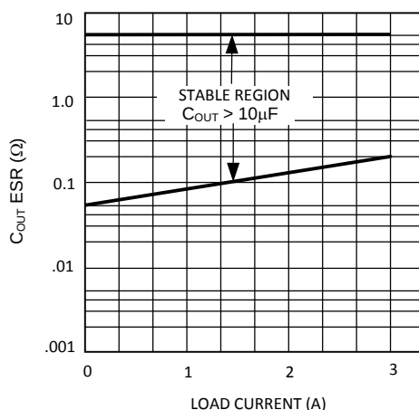
Figure 28. ESR Curve for C_{OUT} (with 10 \mu F Tantalum Input Capacitor)
