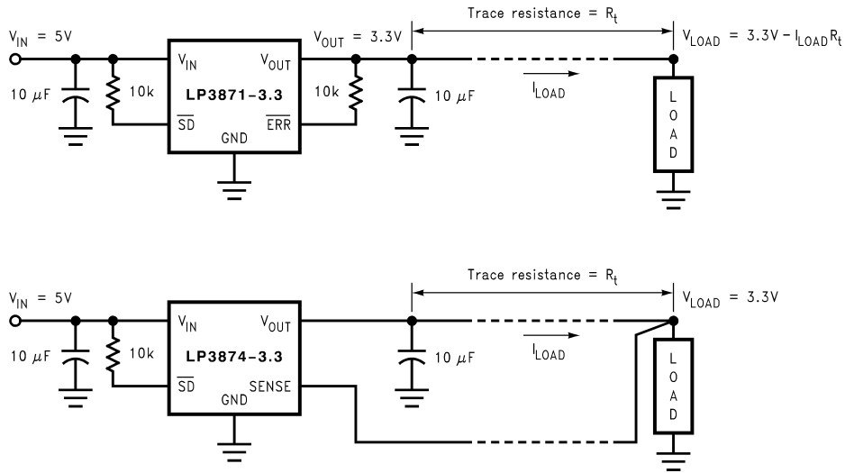
FIGURE 2. Improving remote load regulation using LP3874
