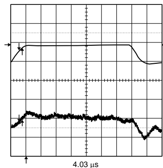
Line Transient Response V_{IN} = 3, 3.6 \text{ V}, V_{OUT} = 1.2 \text{ V}, 250 \text{ mA load}
