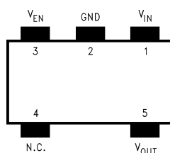
Figure 1. Top View See Package Number DBV
