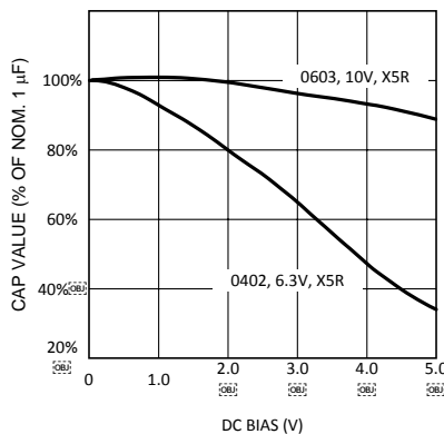
Figure 43. Graph Showing A Typical Variation in Capacitance vs DC Bias
