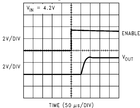
T ON @ MODE = 1.8V, C OUT = 4.7μF, I L = 150mA
