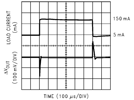
Load Transient Response @ V_{IN} = 3.1V , C_{OUT} = 1\mu F
