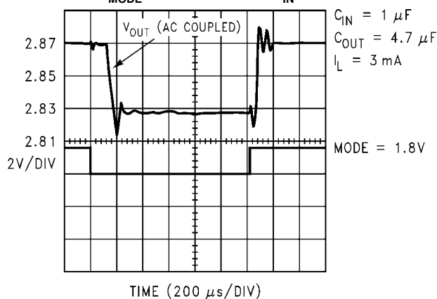
T_{MODE} Measurement @ V_{IN} = 3.6V
