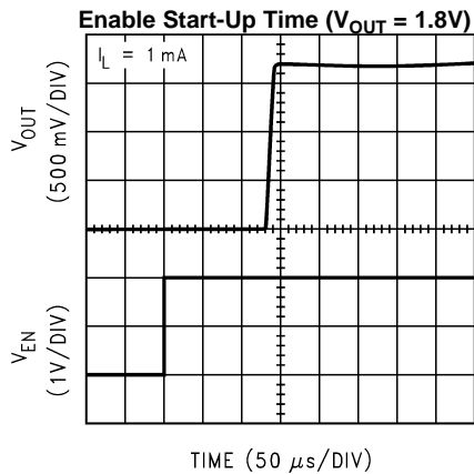
TIME (50 \mu\text{s} /DIV) Figure 13.
