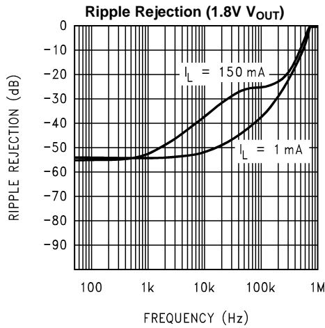
FREQUENCY (Hz) Figure 11.
