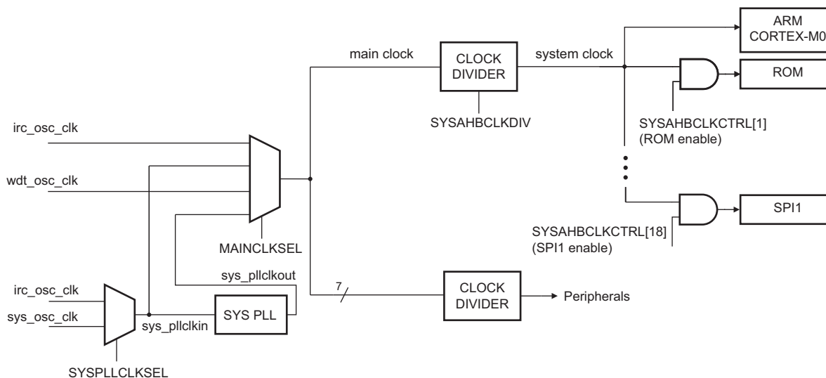
Fig 12. LPC111x/102/202/302 clock configuration for power API use
