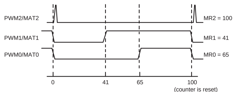
Fig 73. Sample PWM waveforms with a PWM cycle length of 100 (selected by MR2) and MAT2:0 enabled as PWM outputs by the PWCM register.
