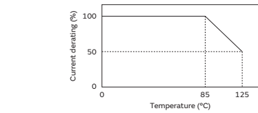
Derating of Rated Current
