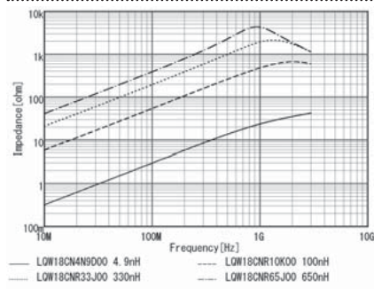
Impedance-Frequency Characteristics (Typ.)
