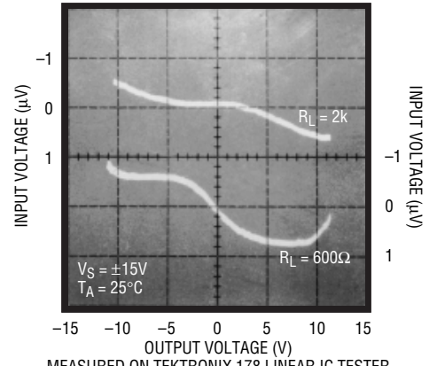
Voltage Gain, R_L = 2k and 600\Omega
