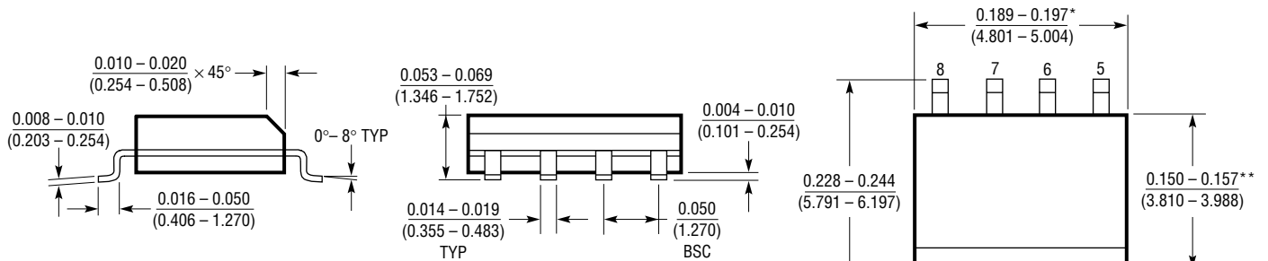
S8 Package 8-Lead Plastic Small Outline (Narrow .150 Inch) (Reference LTC DWG # 05-08-1610)
