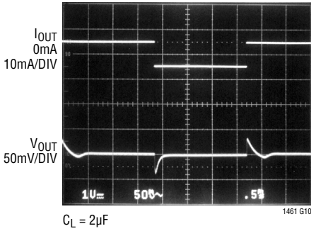
2.5V Transient Response to 10mA Load Step
