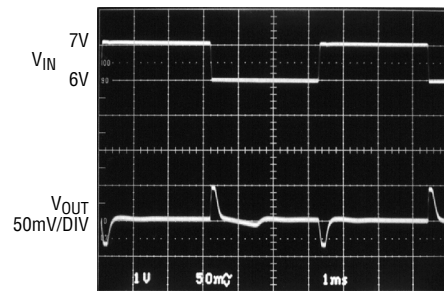
5V Line Transient Response
