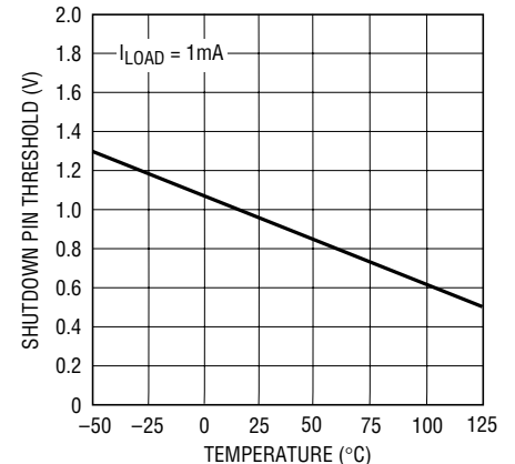
Shutdown Pin Threshold (On-to-Off)
