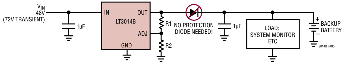
LT3014B Telecom Application
