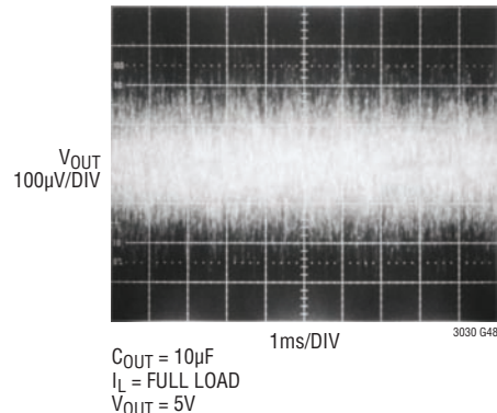
10Hz to 100kHz Output Noise, C_{BYP} = 100\text{pF}
