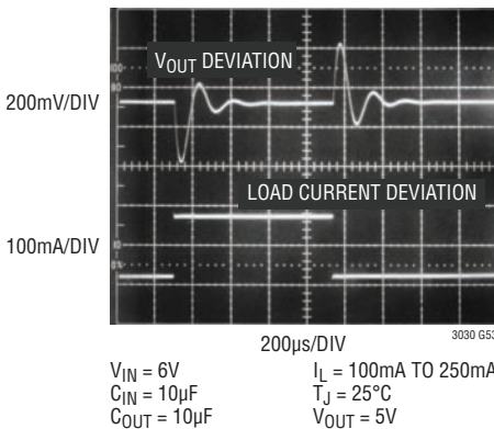
OUT2 Transient Response C_{BYP} = 0\text{pF}
