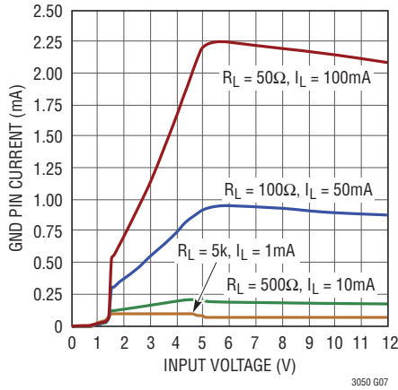
GND Pin Current LT3050-5
