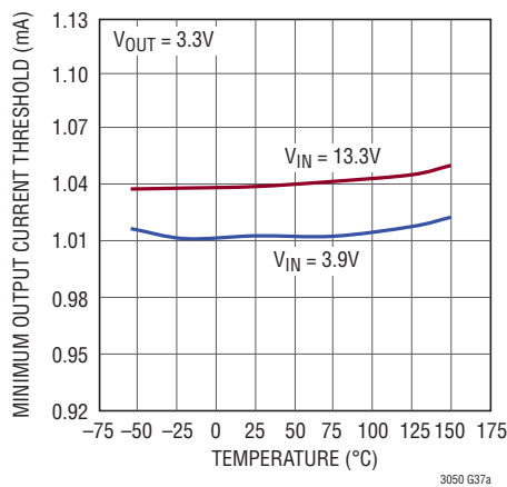
Minimum Output Current Threshold R_{I\text{MIN}} = 110\text{k}
