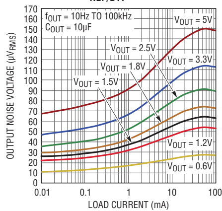
RMS Output Noise vs Load Current C_{\text{REF/BYP}} = 10\text{nF}
