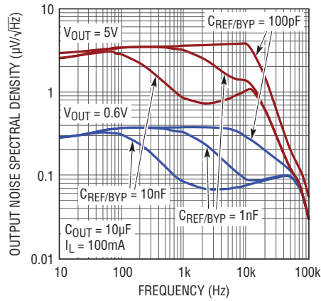
Output Noise Spectral Density vs C_{\text{REF/BYP}} , C_{\text{FF}} = 0
