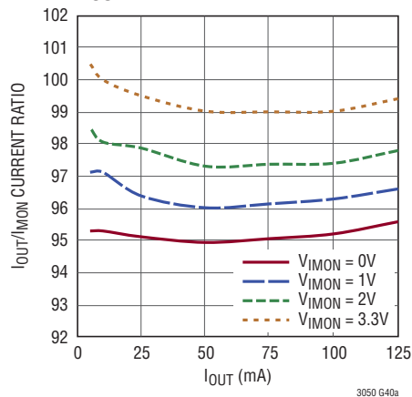
I_{\text{OUT}}/I_{\text{MON}} Current Ratio V_{\text{OUT}} = 3.3\text{V} , V_{\text{IN}} = 3.9\text{V}
