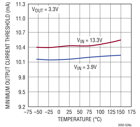
Minimum Output Current Threshold R_{I\text{MIN}} = 11.3\text{k}
