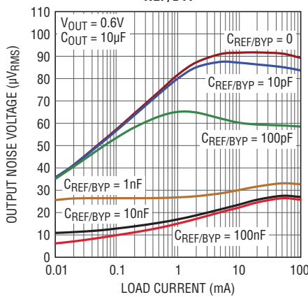
RMS Output Noise vs Load Current vs C_{\text{REF/BYP}}
