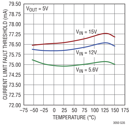
External Current Limit R_{I\text{MAX}} = 1.5\text{k}
