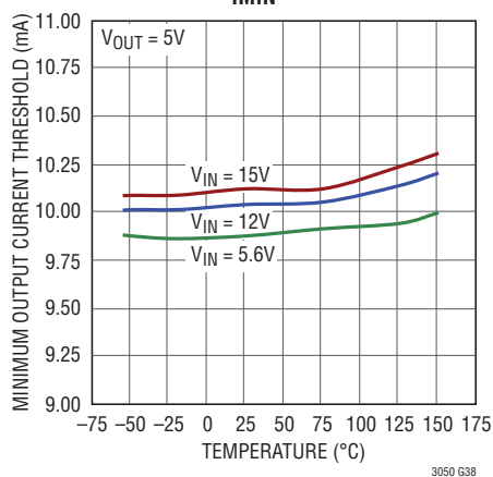
Minimum Output Current Threshold R_{I\text{MIN}} = 11.3\text{k}
