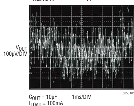
5V 10Hz to 100kHz Output Noise C_{\text{REF/BYP}} = 10\text{nF} , C_{\text{FF}} = 0
