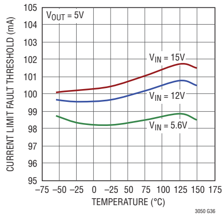
External Current Limit R_{I\text{MAX}} = 1.15\text{k}
