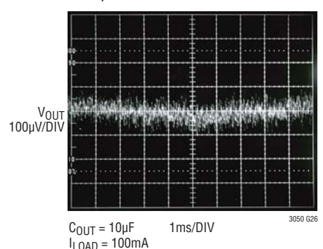
5V 10Hz to 100kHz Output Noise C_{\text{REF/BYP}} = 10\text{nF} , C_{\text{FF}} = 10\text{nF}
