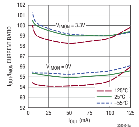
I_{\text{OUT}}/I_{\text{MON}} Current Ratio V_{\text{OUT}} = 3.3\text{V} , V_{\text{IN}} = 3.9\text{V}
