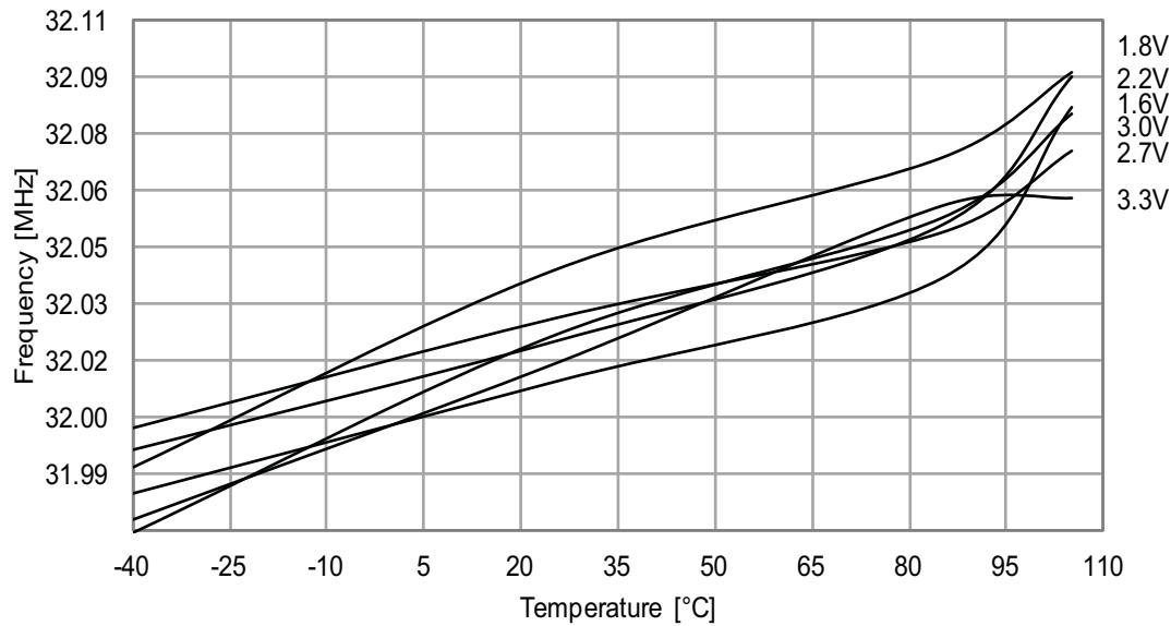
Figure 37-71. 32MHz Internal Oscillator Frequency vs. Temperature DFLL enabled, from the 32.768kHz internal oscillator.
