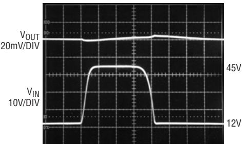
Transient Response (Load Dump)
