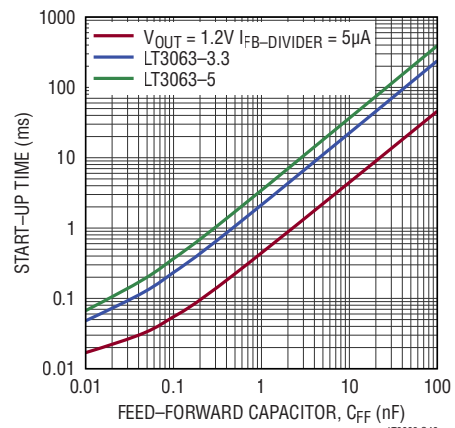
Start-Up Time vs CFF
