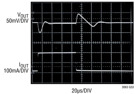
5V Transient Response C_{FF} = 10nF, I_{OUT} = 20mA to 200mA
