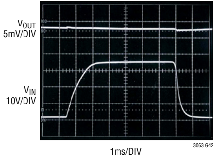
Transient Response, V_{OUT} = 5\text{V} Load Dump, V_{IN} = 12\text{V} to 45\text{V}
