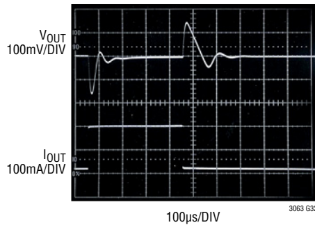
5V Transient Response C_{FF} = 0, I_{OUT} = 20mA to 200mA
