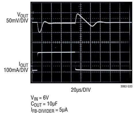
5V Transient Response C_{FF} = 10\text{nF} , I_{OUT} = 20\text{mA} to 200\text{mA}
