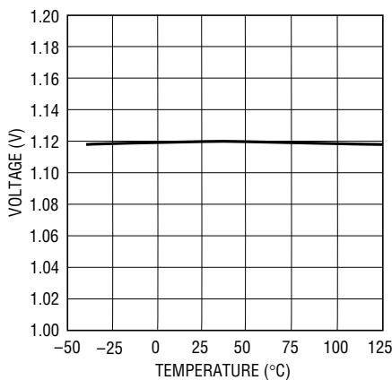
PGFB Threshold
