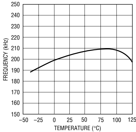
Oscillator Frequency
