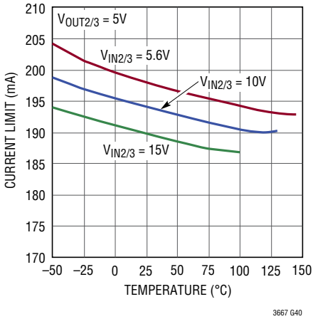
LDOs: External Current Limit, REN/LIM = 1.54k
