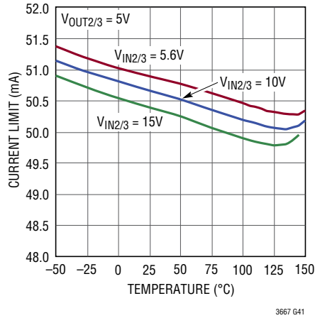
LDOs: External Current Limit, REN/LIM = 6.19k
