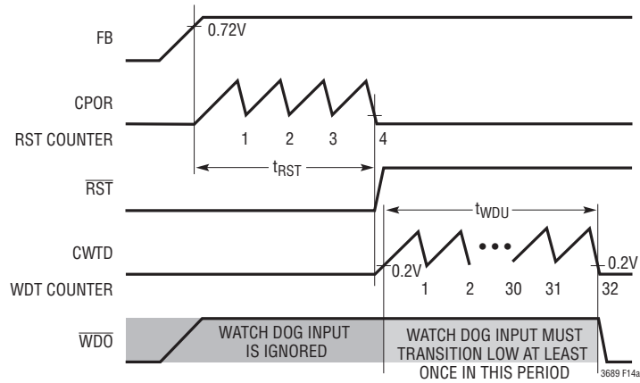
(14a) \bar{W}/T = High. The First Valid Negative Edge on WDI Must Occur Before the Watchdog Timer Expires
