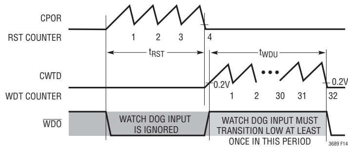
(14c) \bar{W}/T = Low. Restart Sequence After a Timing Fault
