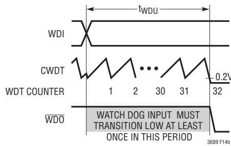
(14b) \bar{W}/T = High. Subsequent Edges Must Occur Before the Timer Expires
