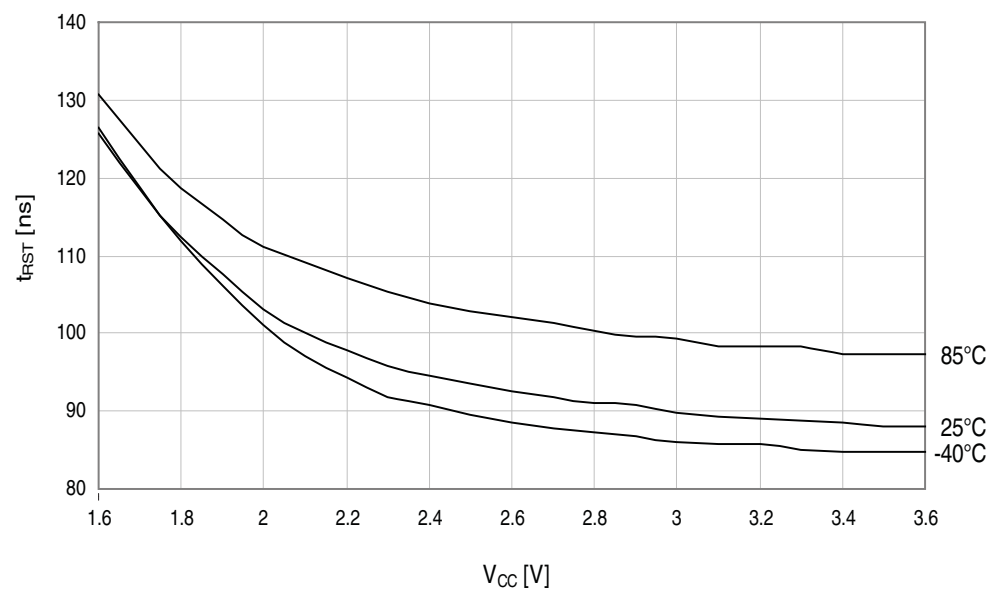
Figure 37-51.Minimum Reset pin pulse width vs. V_{CC} .
