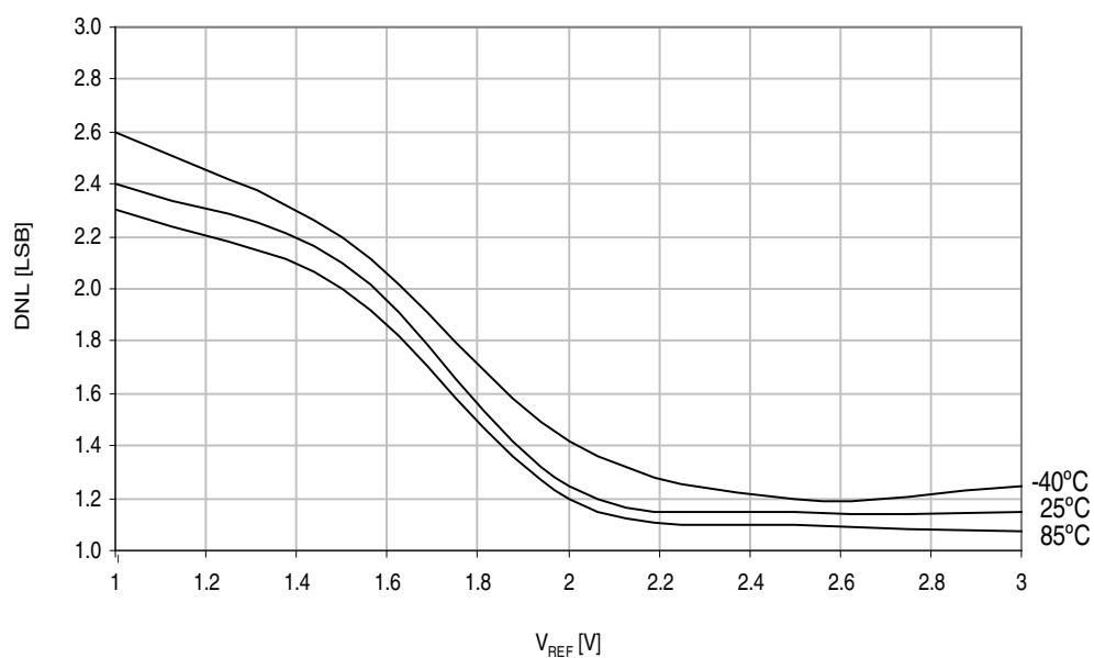
Figure 37-27. ADC DNL vs. V_{REF} .
