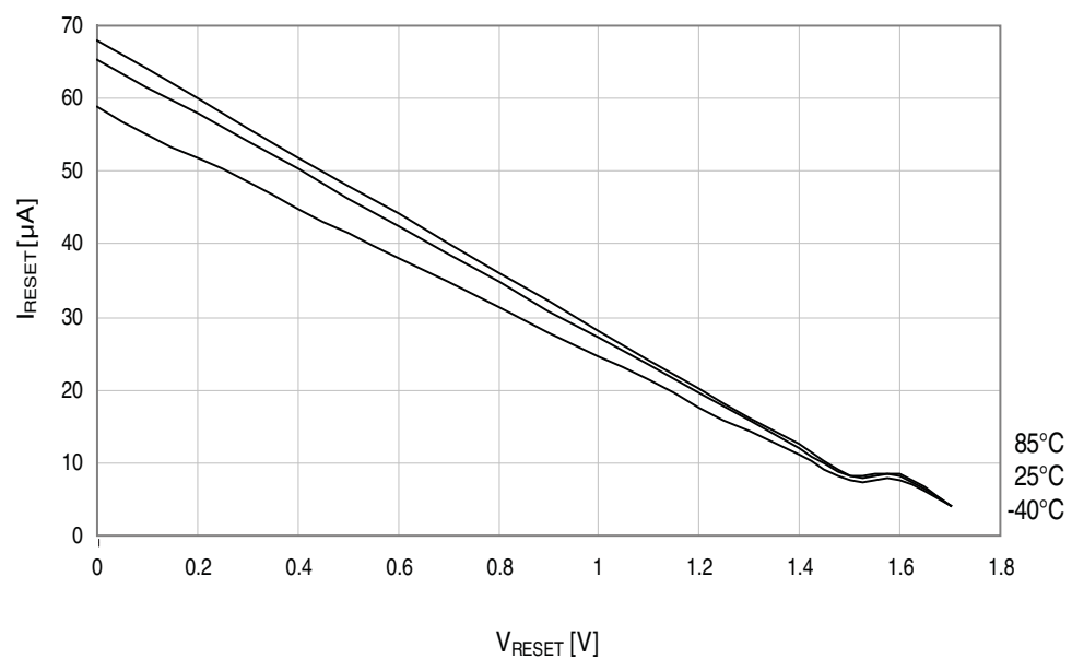
Figure 37-52.Reset pin pull-up resistor current vs. reset pin voltage. V_{CC} = 1.8V .
