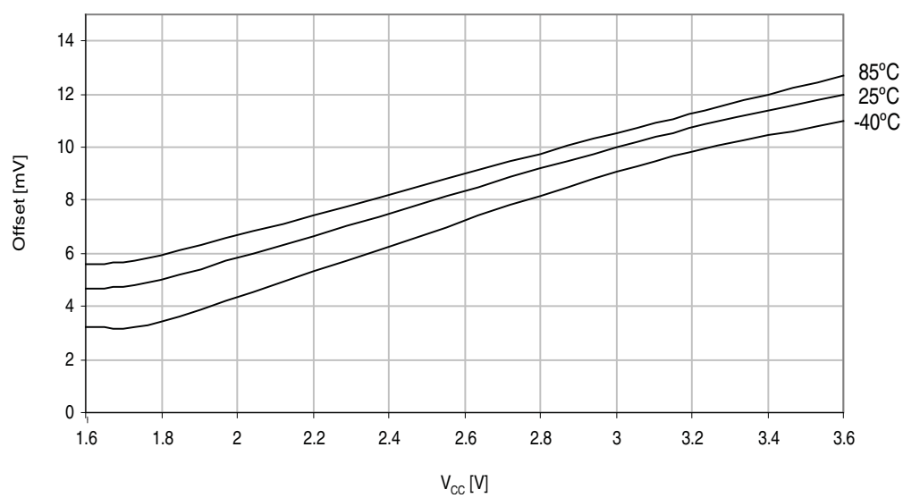
Figure 37-28. ADC Offset vs. V_{CC} .
