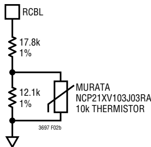
Figure 2b. R_{\text{CBL}} Resistor Network for Matching Copper Wire Temperature Coefficient
