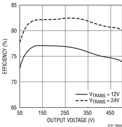
Efficiency
