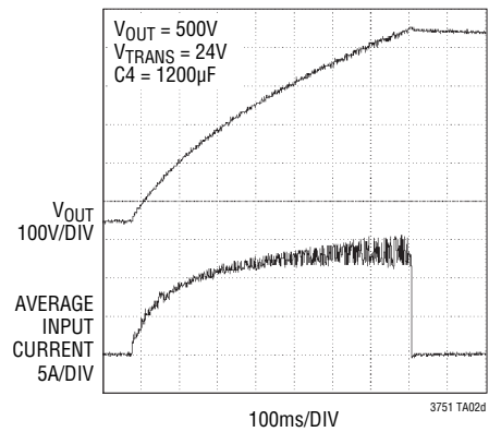
Charging Waveform
