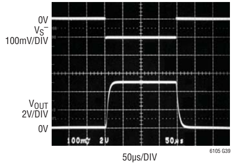
Step Response V_{SENSE} = 0V to 100mV , C_L = 1000pF , V_{S^+} = 0V
