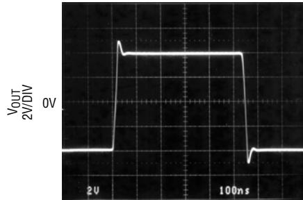
Large-Signal Response
