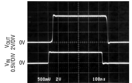
Output-Overload Recovery
