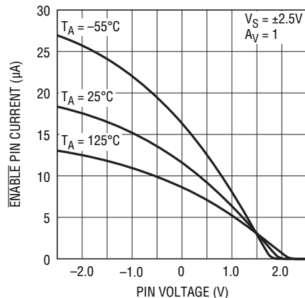
ENABLE Pin Current vs ENABLE Pin Voltage
