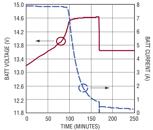
Charge Profile
