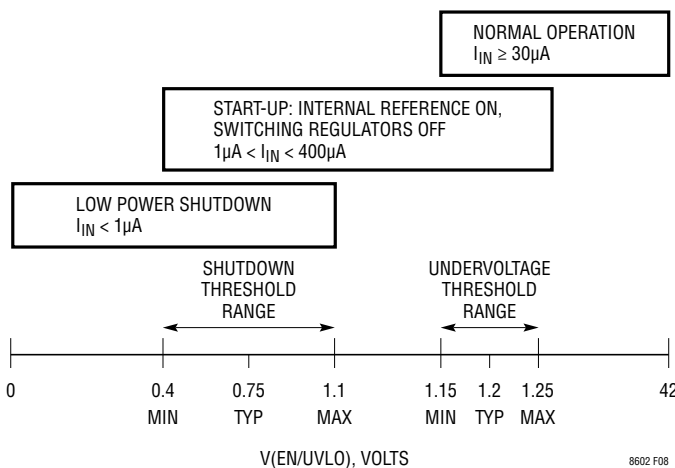
Figure 8. EN/UVLO Thresholds
