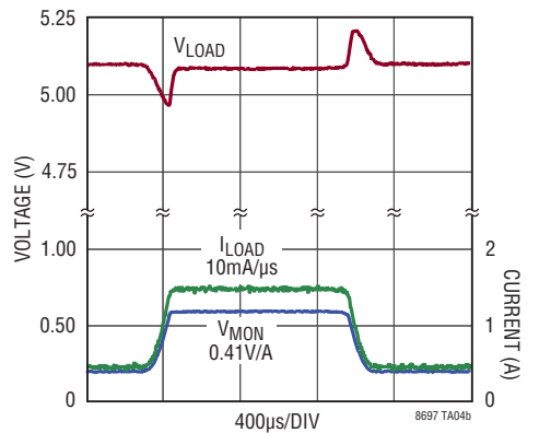
Transient Response 0.5A to 1.5A Load Step
