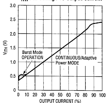
V_{Ith} Pin Voltage vs Output Current
