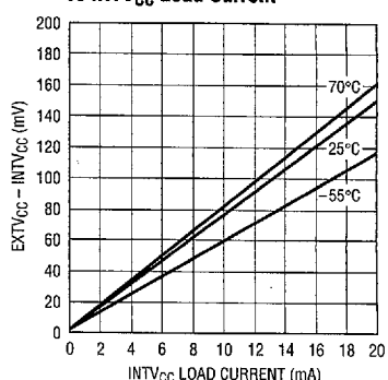
EXTV_{CC} Switch Drop vs INTV_{CC} Load Current
