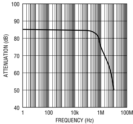
Reference Feedthrough
