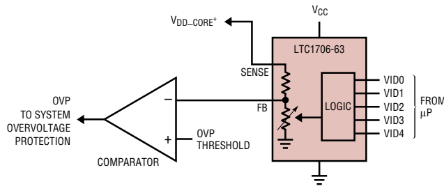
2-Phase 12V Input, 1.025V to 1.4125V/45A Max Power Supply (LTC3819) with Adjustable Overvoltage Protection (LTC1706-63)
