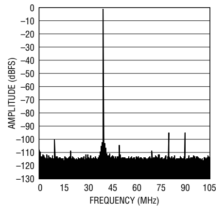
64k Point FFT, f_{IN} = 170.0\text{MHz} , -1\text{dBFS} , \text{PGA} = 1 , Dither On
