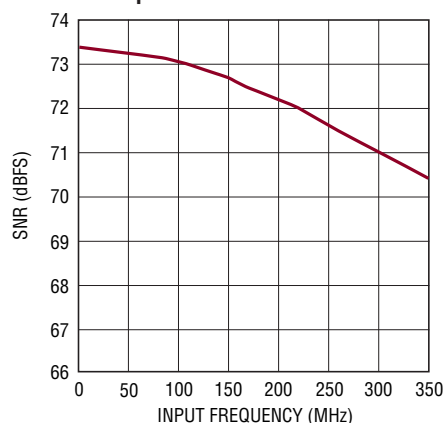
LTC2264-14: SNR vs Input Frequency, -1\text{dBFS} , 2\text{V} Range, 40\text{Mps}
