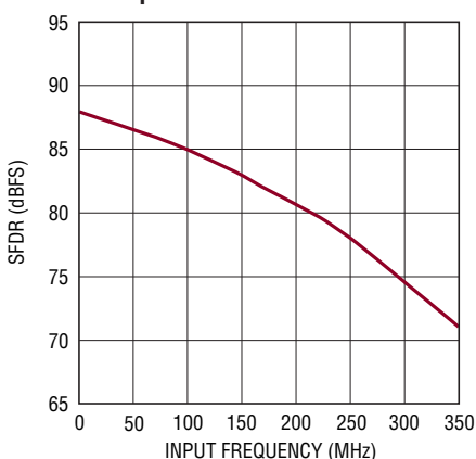
LTC2264-14: SFDR vs Input Frequency, -1\text{dBFS} , 2\text{V} Range, 40\text{Mps}
