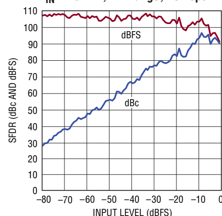
LTC2264-14: SFDR vs Input Level, f_{IN} = 70\text{MHz} , 2\text{V} Range, 40\text{Mps}
