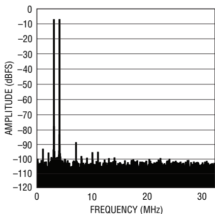
LTC2265-14: 8k Point 2-Tone FFT, f_{IN} = 68\text{MHz} , 69MHz, -1dBFS, 65Mpsps
