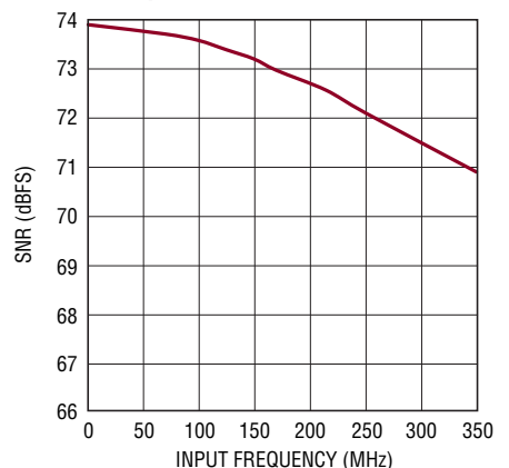
LTC2265-14: SNR vs Input Frequency, -1dBFS, 2V Range, 65Mpsps
