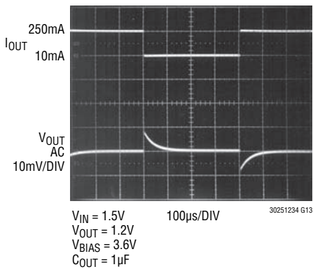
Transient Response
