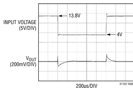
Fast (10μs) Cold Crank Line Transient, V_{IN} = 13.8V to 4V
