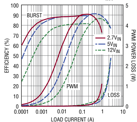
V_{OUT} = 3.3\text{V} Efficiency and Power Loss vs Load Current from V_{IN1}
