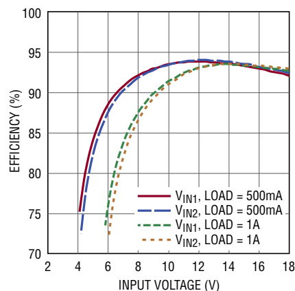
5V OUT Efficiency vs V_{IN1} or V_{IN2} Voltage with 500mA and 1A Load Current
