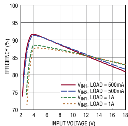
3.3V OUT Efficiency vs V_{IN1} or V_{IN2} Voltage with 500mA and 1A Load Current
