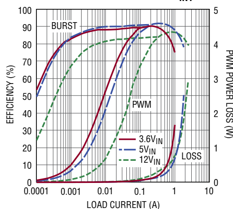
V_{OUT} = 5\text{V} , Efficiency and Power Loss vs Load Current from V_{IN1}
