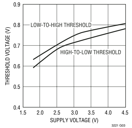
\overline{\text{SHDN}} Threshold Voltage vs Supply Voltage
