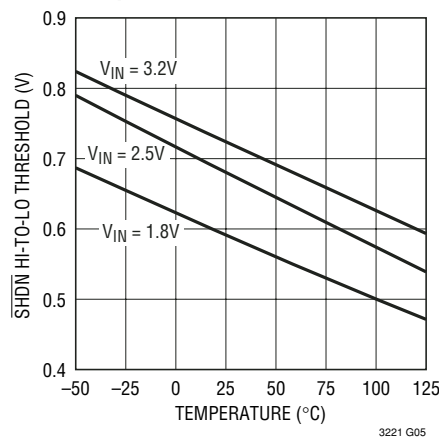
\overline{\text{SHDN}} HI-to-LO Threshold vs Temperature
