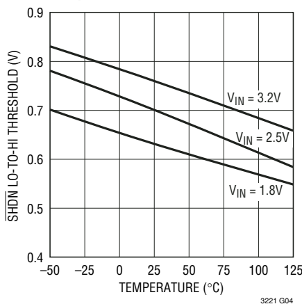
\overline{\text{SHDN}} LO-to-HI Threshold vs Temperature
