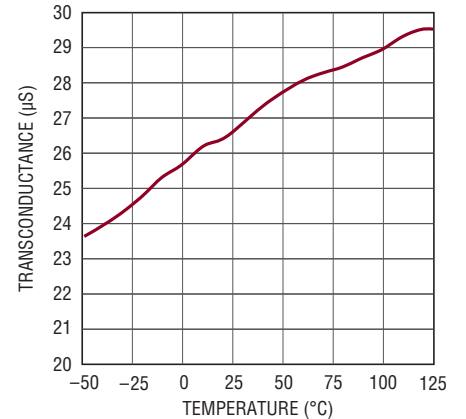
Boost Error Amplifier Transconductance vs Temperature
